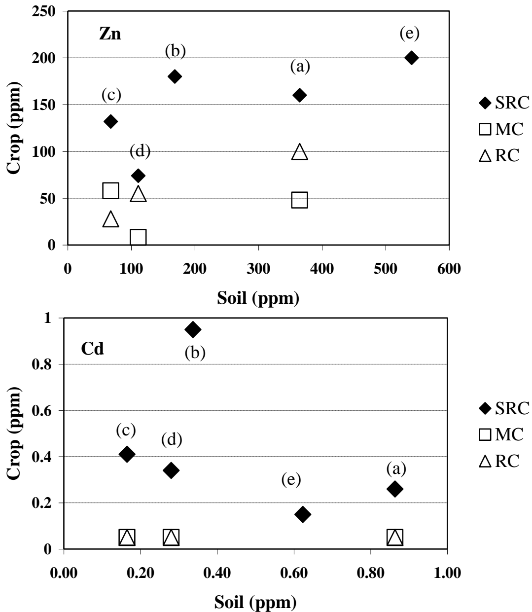
Figure 1. Comparison of Zn and Cd contents of biomass types to average host soils at each energy crop site (a, b, c, d, e). Note: SRC = short rotation coppice, MC = miscanthus, RC = reed canarygrass.
